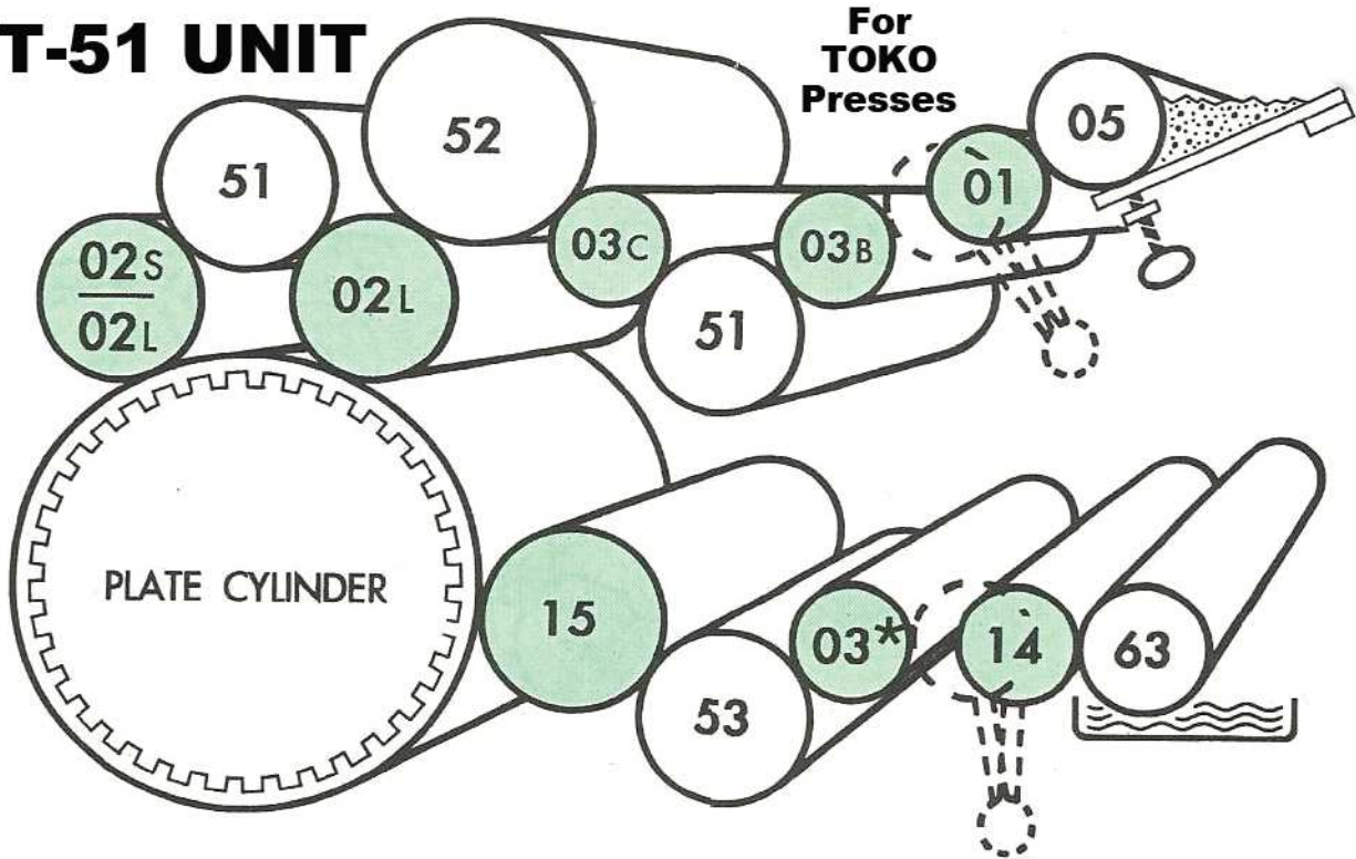
TOWNSEND T-51 on Toko 4700, 4750CD, R1
