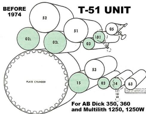
Townsend T-51 On AB Dick 350 (1973 & Earlier - Old Style T-51 With 2 Ink Oscillators)
