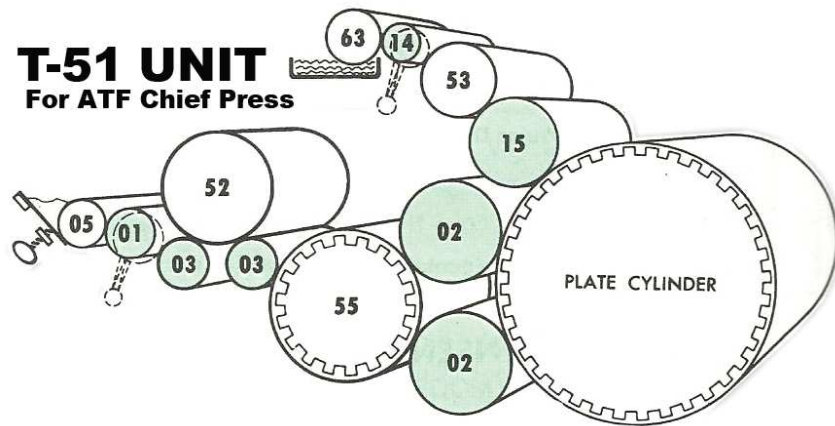
TOWNSEND T-51 on ATF Chief 15, 17
