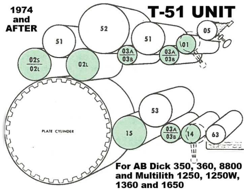
Townsend T-51 On AB Dick 350 (1974 & After - New Style T-51 With 3 Ink Oscillators), AB Dick 360
