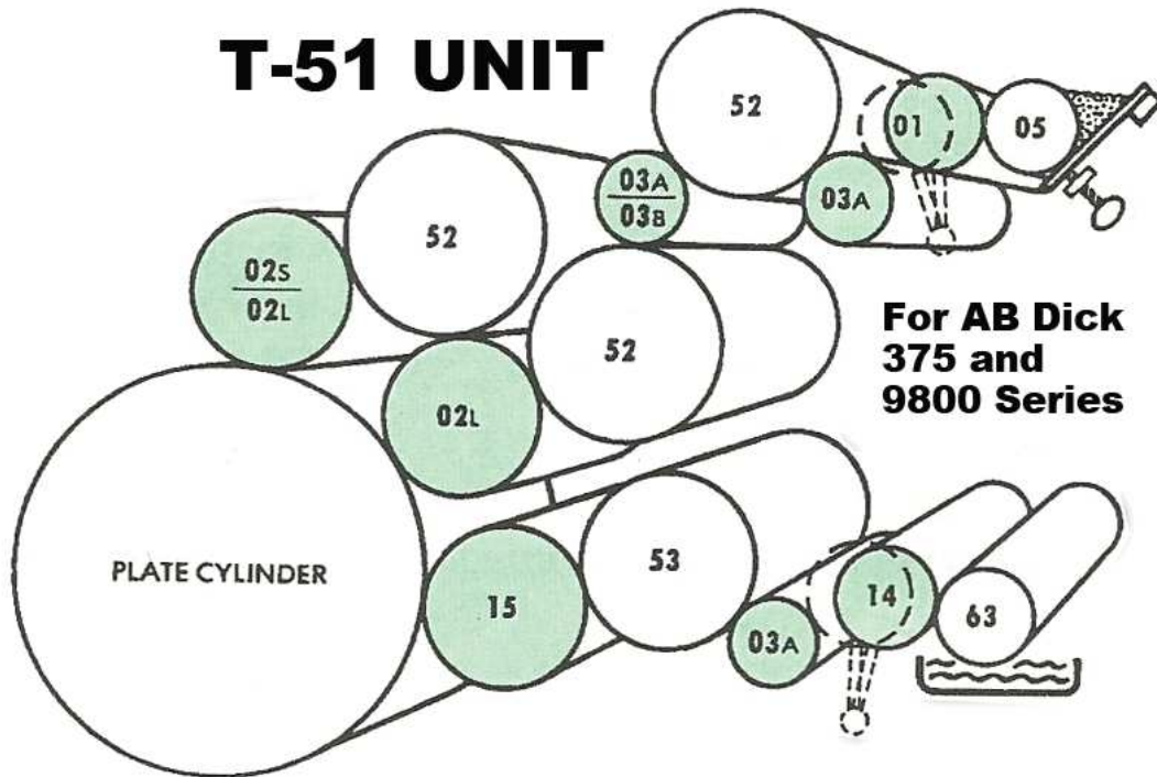
TOWNSEND T-51 on AB Dick 375, 9800; Multilith 1360, 1650
